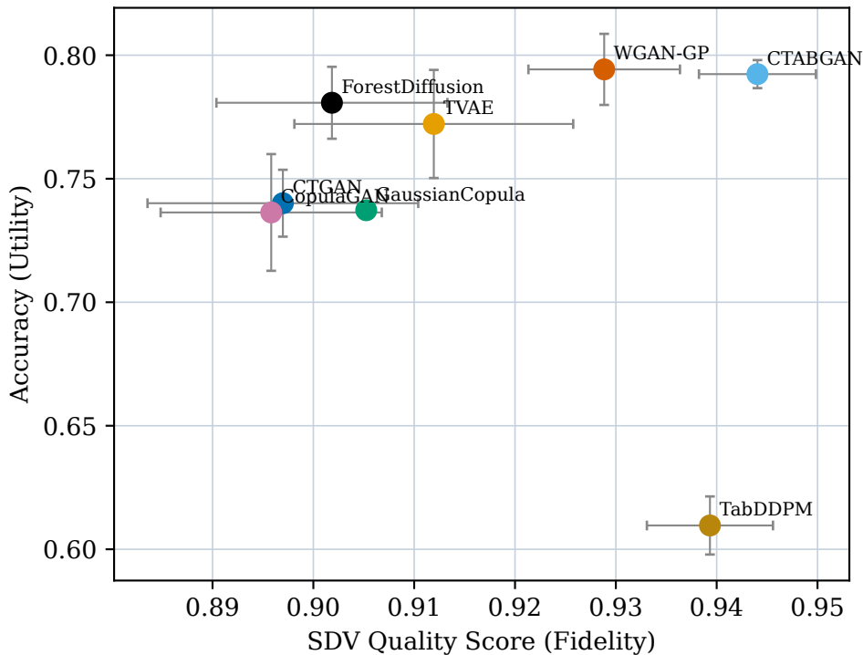
MAGIC Gamma: SDV Quality Score (Fidelity) vs Accuracy (Utility)
